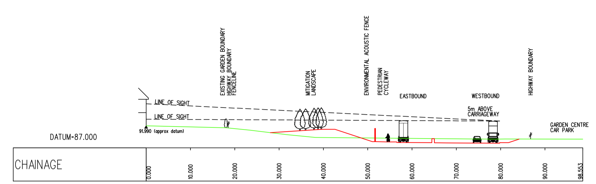
NOTE: Height of existing trees to be confirmed SECTION 2 - 2
